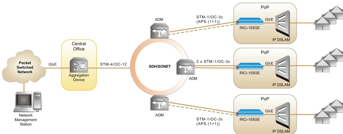
Figure 1. IP DSLAM Backhauling
