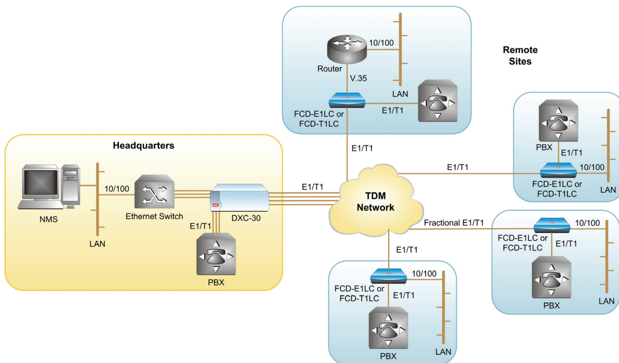
Figure 1. Extended Ethernet Management over E1/T1 Network
