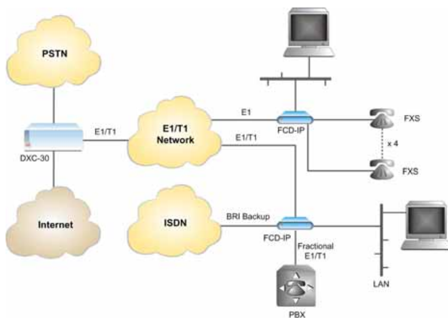
Figure 1. Bundled Services
