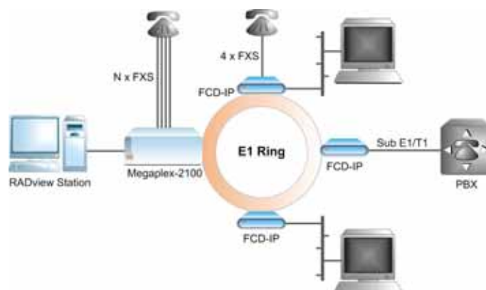
Figure 3. FCD-IP in an E1 Ring Topology
